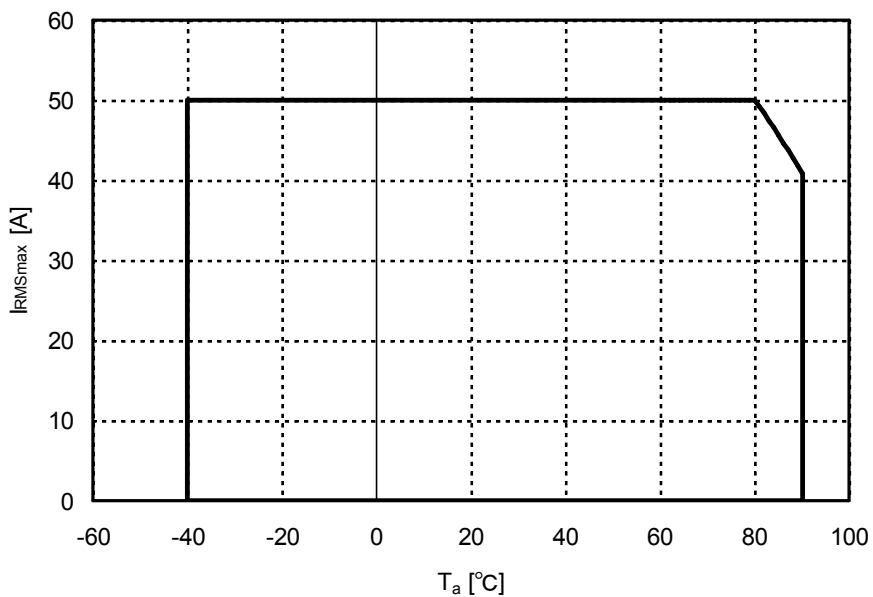
Figure 4. Primary current derating curve of CQ-2065
