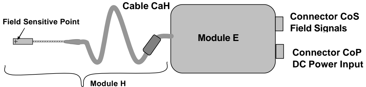
Figure 1: Structure of a SENIS high-accuracy Hall Magnetic Field Transducer
