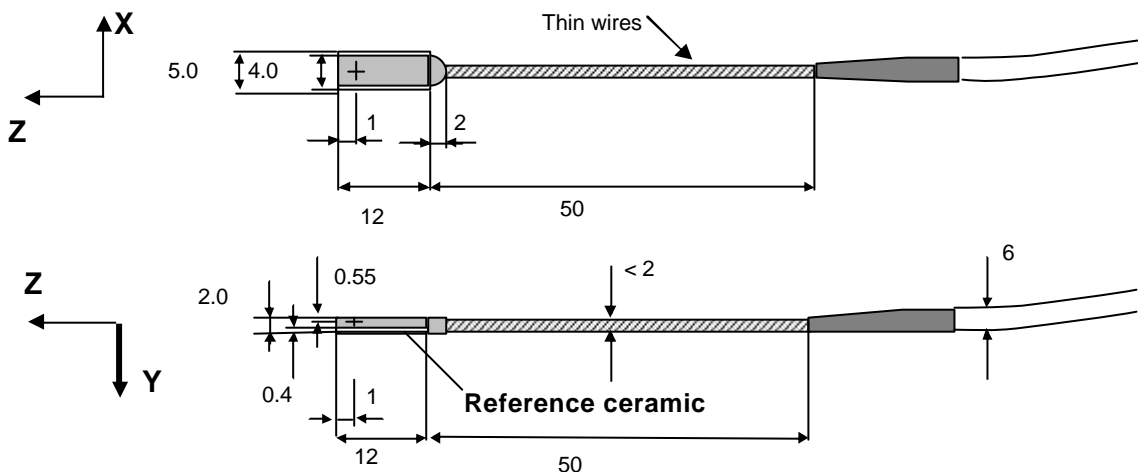
Figure 2: Probe dimensions and position of the active zone for the Single-Axis Magnetic Field Hall Transducer (module H). All measures are in millimeters.
