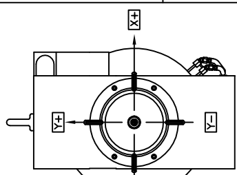
MAGNET SIDE VIEW
